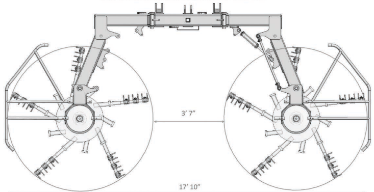
NARROW SETTING, ARMS OUT, STANDARD RAKE BARS
