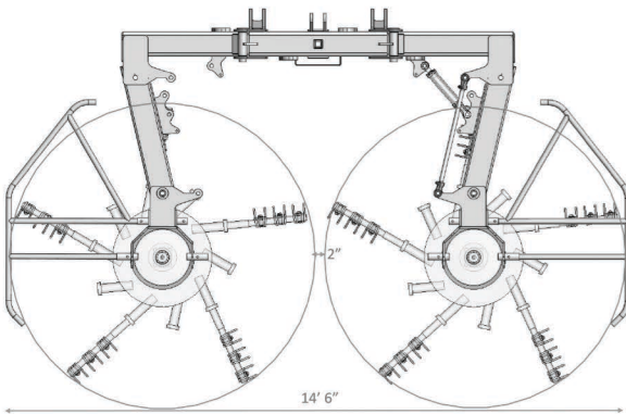
NARROW SETTING, ARMS IN, STANDARD RAKE BARS
