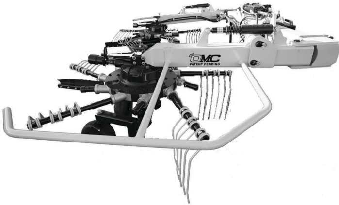
NARROW SETTING, ARMS IN, STANDARD RAKE BARS
