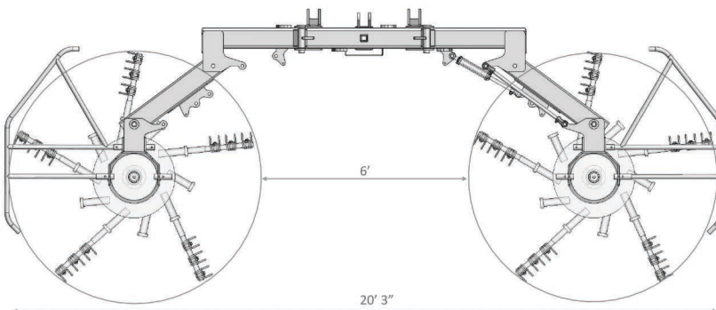
WIDE SETTING, ARMS OUT, STANDARD RAKE BARS
