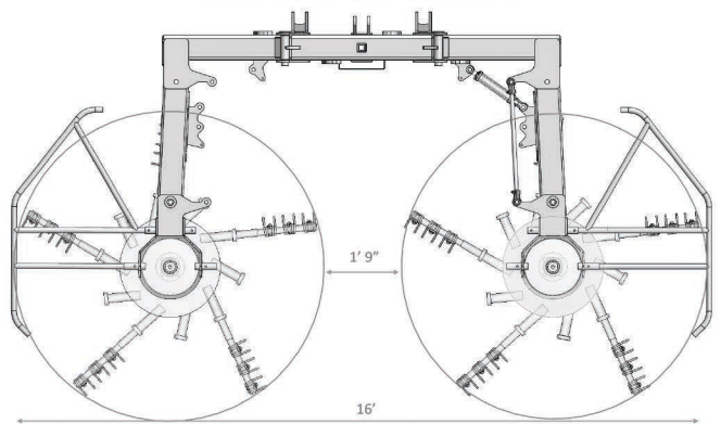
WIDE SETTING, ARMS IN, STANDARD RAKE BARS
